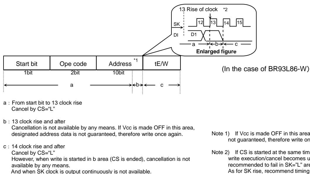
Figure 41. ERASE, ERAL cancel available timing
