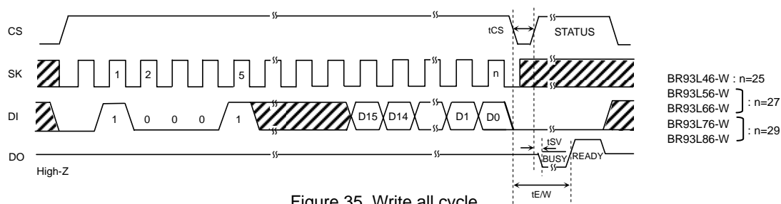
Figure 35. Write all cycle
