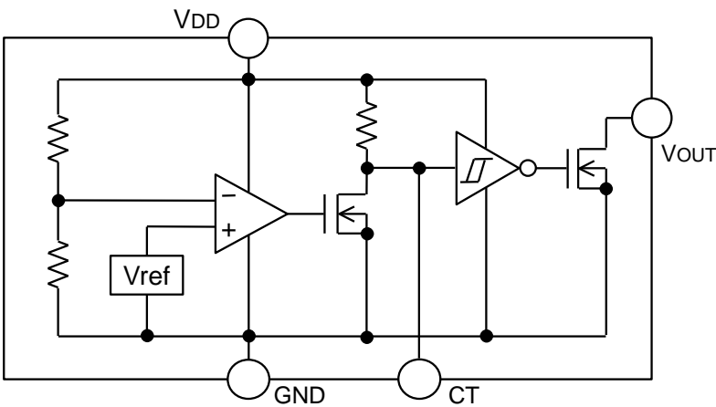
Fig.1 BD52xx Series
