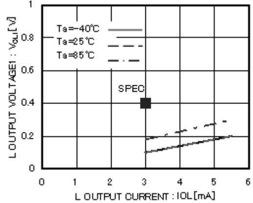
Figure 11. 'L' Output Voltage1 V_{OL1}-I_{OL}(V_{CC1}=3.0V) (SDA1)
