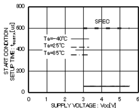
Figure 29. Start Condition Setup Time t_{SU:STA}
