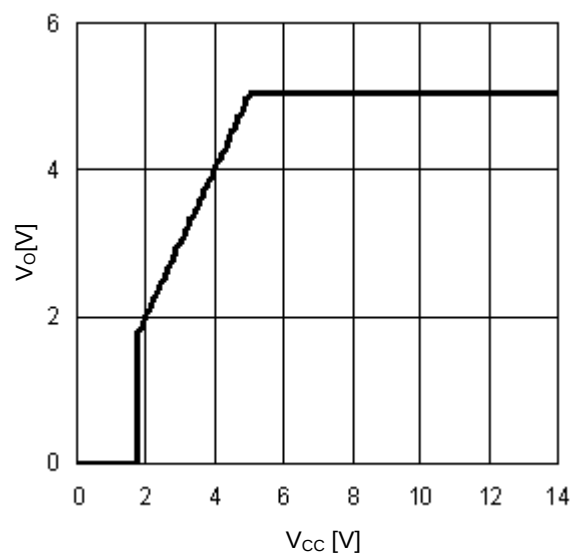
Figure 15. V_{cc}-V_o ( I_o=0mA )
