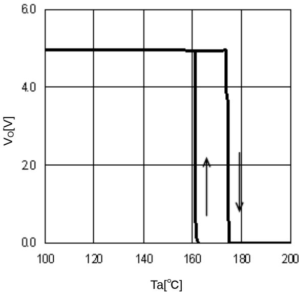
Figure 16. TSD ( I_o=0mA )
