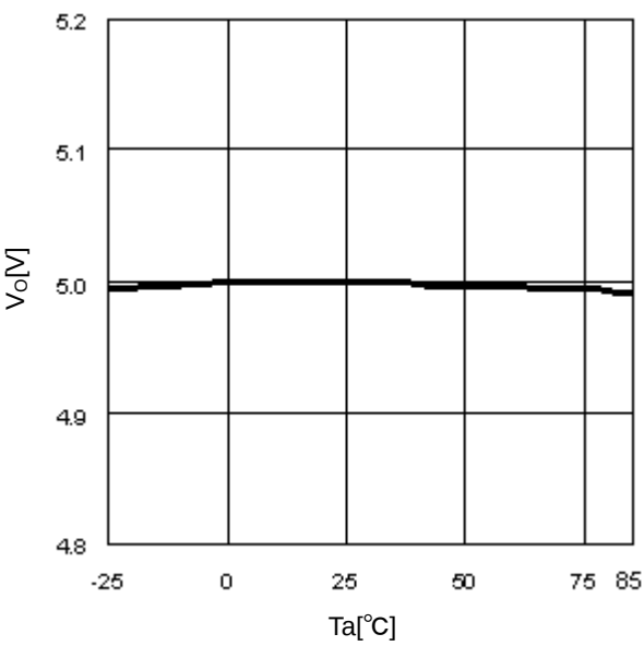
Figure 9. T_a-V_O ( I_O=0mA )
