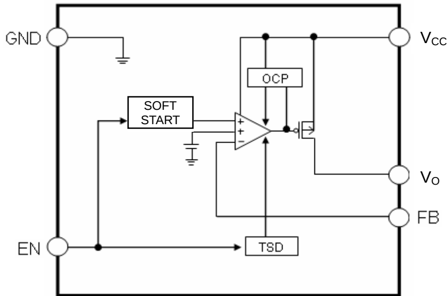
Figure 1. Block Diagram
