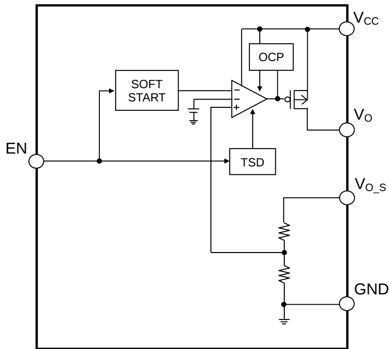
Figure 2. Block Diagram
